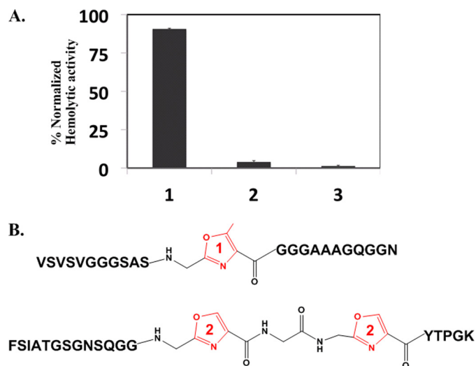
FIGURE 5. Hemolytic activity of MBP-CloxA T46A and structures of identified PTM peptides. A , synthetase reactions using MBP-CloxA T46A and SagB/CloxC/CloxD. Hemolytic activity was normalized against a Triton X-100 positive control. Lane 1 , wt CloxA and SagB/CloxC/CloxD; lane 2 , SagB/CloxC/CloxD only; lane 3 , CloxA T46A and SagB/CloxC/CloxD. B , peptide 1, CLS peptide containing a methyloxazole at position Thr 46 ; peptide 2, SLS peptide containing two oxazoles at positions Ser 46 and Ser 48 .
