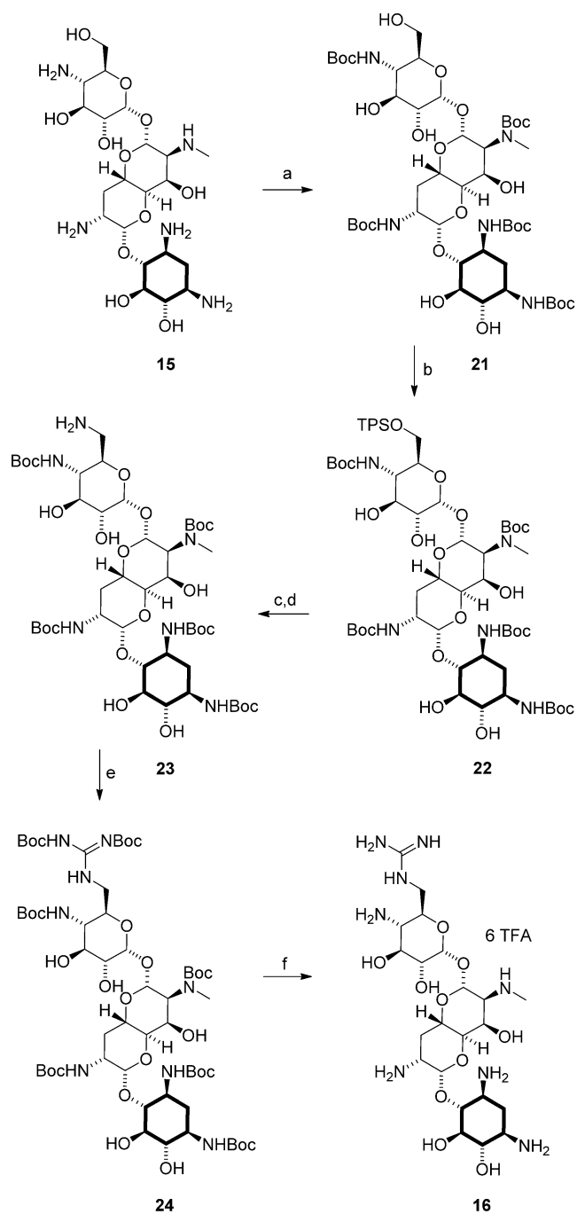
Scheme 2. 6''-Deoxy-6''-guanidinoapramycin synthesis. Reagents and conditions: a) \text{Boc}_2\text{O} , \text{Et}_3\text{N} , \text{H}_2\text{O} , DMF, 55^\circ\text{C} , 8 h, 92%; b) TPSCl, pyridine, RT, 1.5 days, 31%; c) \text{NaN}_3 , DMF, 55^\circ\text{C} , 2 days; d) Pd/C, \text{H}_2 , MeOH, RT, overnight, 80% (two steps); e) 1,3-di-Boc-2-(trifluoromethylsulfonyl)guanidine, \text{Et}_3\text{N} , \text{CH}_2\text{Cl}_2 , MeOH, RT, 3 days, 74%; f) TFA, TIPS, \text{CH}_2\text{Cl}_2 , RT, 2 h, 78%.
